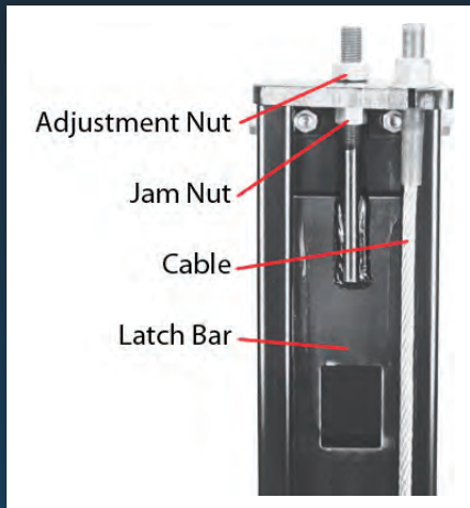
Exclusive adjustable lock ladder leveling system
